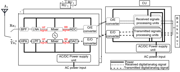
Fig. 2: Power-consuming units in a C-RAN architecture (DL).
