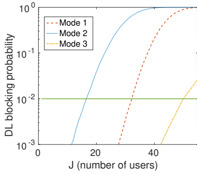
Fig. 4: DL blocking probability with P_t = -13 dBm per RB.
