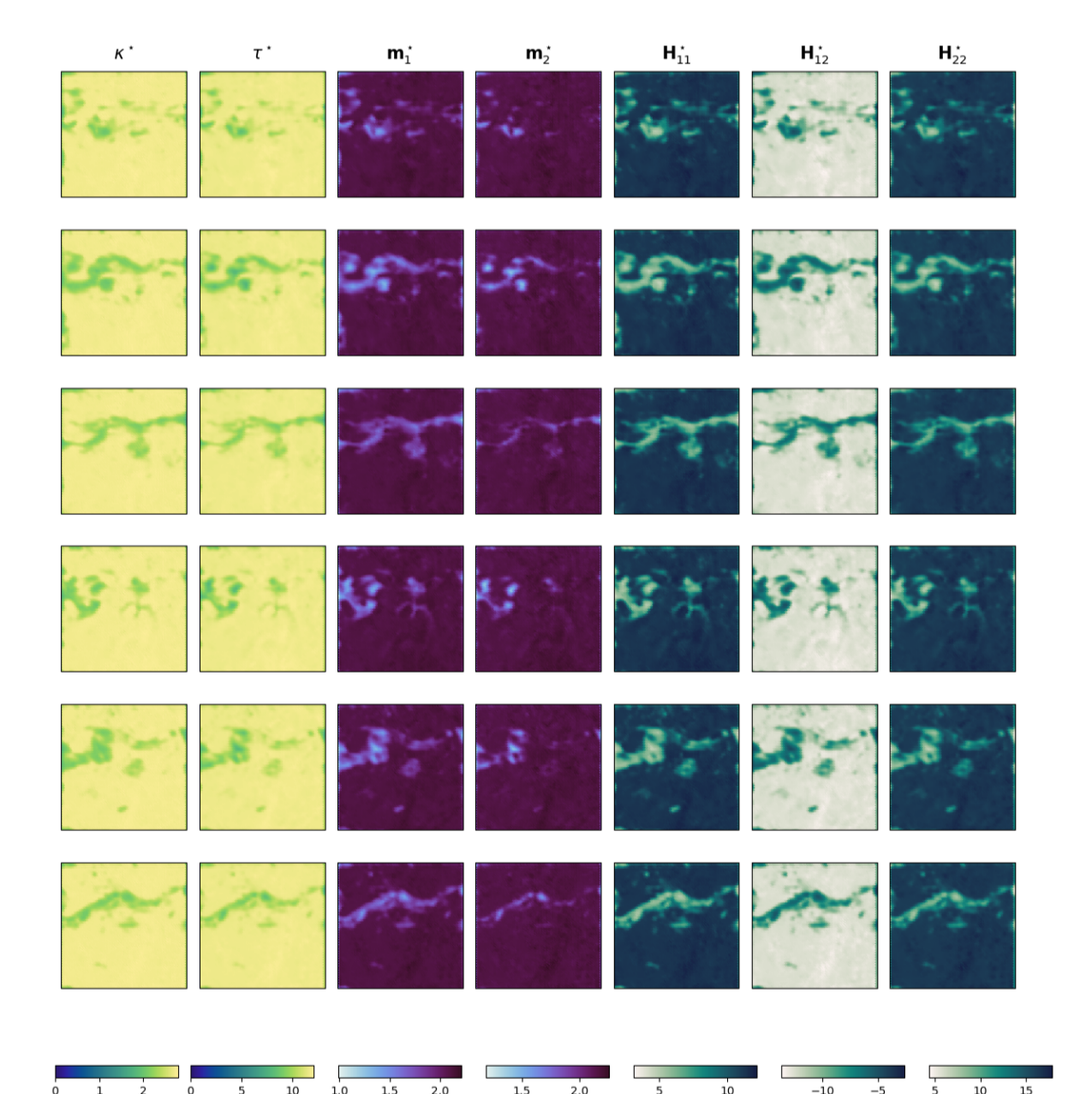
Figure 4: Parameter estimation of the SPDE prior in the neural scheme along the 2020 ODC 42 days test period and every 6 days. From left to right: \kappa , \tau (variance regularization), \mathbf{m}^1 , \mathbf{m}^2 (advection fields), \mathbf{H}^{1,1} , \mathbf{H}^{1,2} and \mathbf{H}^{2,2} (diffusion tensor).
