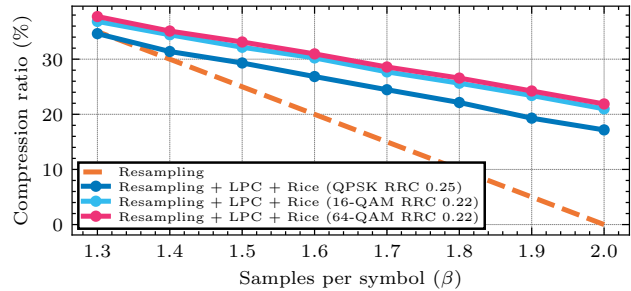
Fig. 3: Graph depicting the progression of the overall compression ratio for several waveforms. Signals are processed using LPC-based compression after resampling. Original signals are sampled with 2 samples per symbol.
