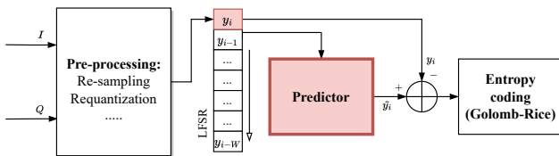
Fig. 2: Classical architecture for compression/decompression scheme using predictive coding.
