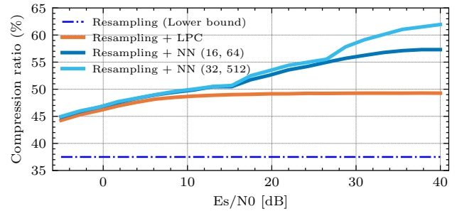
(b) 8-PSK signal shaped with RRC of 0.25 rolloff. Resampling is 1.22 sample per symbol
