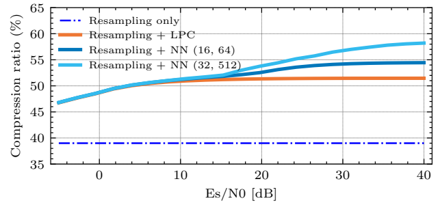
(a) 16-QAM signal shaped with RRC of 0.22 rolloff. Resampling is 1.25 sample per symbol
