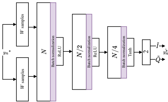
Fig. 4: Architecture of our prediction network
