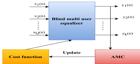
Fig. 2: Multi-user generic equalizer architecture.
