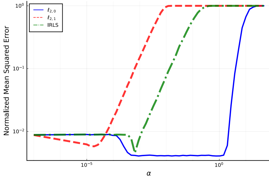
Figure 1: Normalized mean squared error versus regularization parameter \alpha for SNR=40dB
