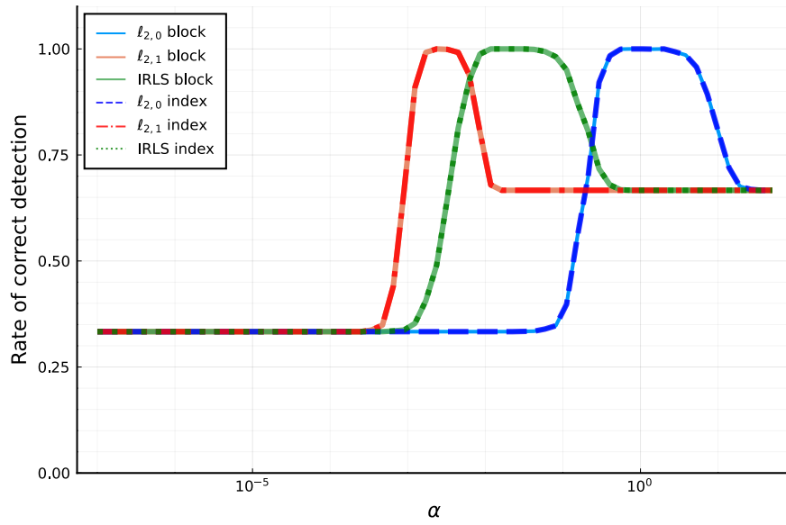
Figure 4: Rate of correct detection versus regularization parameter \alpha for SNR=10dB
