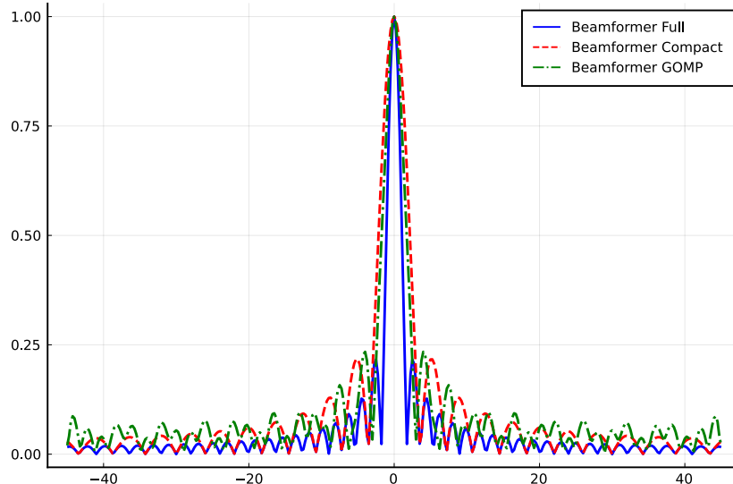
Figure 9: Optimized beamformer with GOMP for direction \theta = 0^\circ (green). Blue and red curves are obtained with the conventional beamformers for 64 and 32 regularly spaced sensors.
