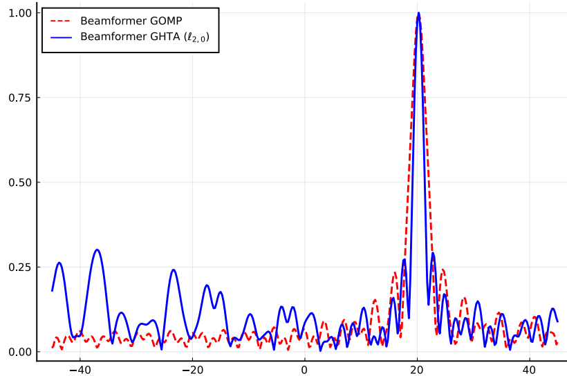
Figure 12: GOMP (red) and GHATA (blue) beamformers of Figures 9 and 10 at about 20^\circ .
