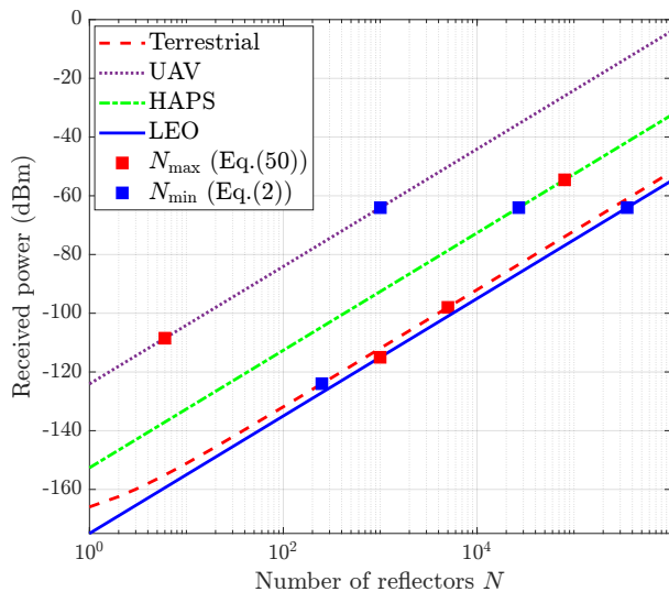
Figure 6. Received power vs. number of reflectors (different platforms; specular reflection paradigm).
