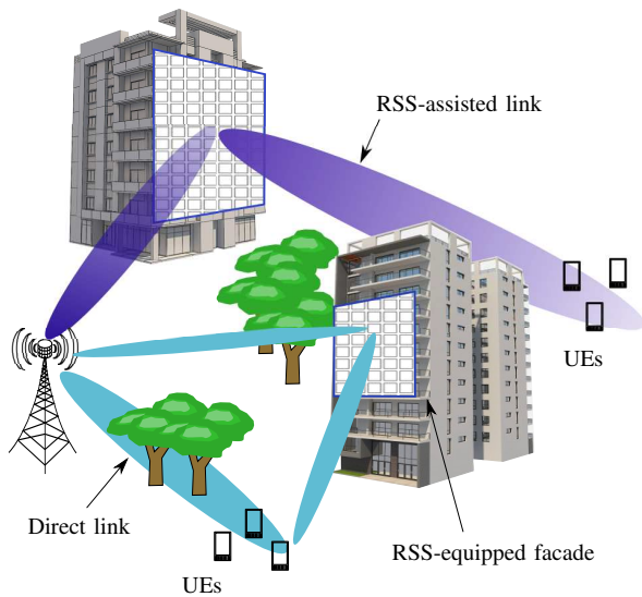
Figure 1. System model of RSS in a terrestrial environment.
