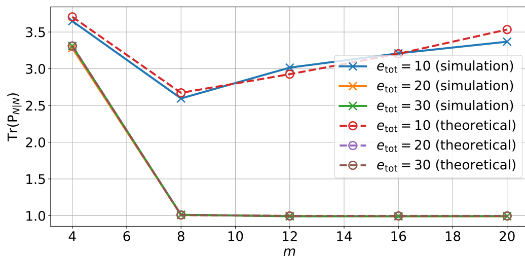
Figure 5. Theoretical and simulated variance of estimation error on the position depending on the number of quantization bits using an unreliable memory for different total energy values e_{\text{tot}} in the case of the large-size example.
