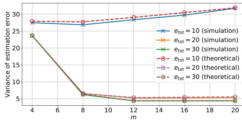
Figure 3. Theoretical and simulated variance of estimation error on the position depending on the number of quantization bits using an unreliable memory for different for different total energy values e_{tot} .
