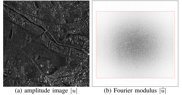
Fig. 1. An example of TerraSAR-X image data. We display in (a) the modulus of a SLC TerraSAR-X image u with size M \times N , and in (b) the modulus of its DFT \hat{u} (low values are displayed in bright and high values are displayed in dark). The Fourier spectrum (b) vanishes outside a rectangular sub-frequency domain \hat{\omega} with size m \times n (delimited by the red dashed line), showing that the image u is oversampled by a factor M/m in the range direction, and by a factor N/n in the azimuth direction.
