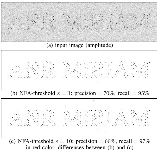
Fig. 11. Target detection by NFA thresholding. A numerical simulation of strong targets mixed in stationary speckle is shown in (a). Targets are detected using Algorithm 3 with two threshold values: \varepsilon = 1 (b) and \varepsilon = 10 (c) corresponding to different trade-offs between a good precision (limited number of false alarms, setting of (b)) and high recall (few targets missed, setting of (c)).
