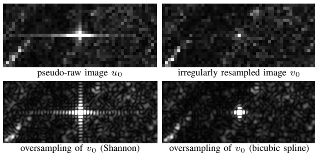
Fig. 7. Re-appearance of the targets sidelobes at the sub-pixelic scale. Thanks to the irregular resampling procedure, the targets induced cardinal sines present in the pseudo-raw image are changed into discrete Diracs in v_0 . Therefore, the targets sidelobes present in u_0 are canceled in v_0 . Unfortunately, we observe a re-appearance of the sidelobes when we oversample v_0 using the Shannon interpolation (see bottom-left image). Even when using a more local interpolation method to oversample v_0 , such as bicubic splines (see bottom-right image), the sidelobes re-appear in the vicinity of the strong targets. This experiment illustrates the inability to manipulate the irregularly resampled image v_0 at the sub-pixelic scale, which restricts its potential use in image analysis algorithms requiring sub-pixelic precision.
