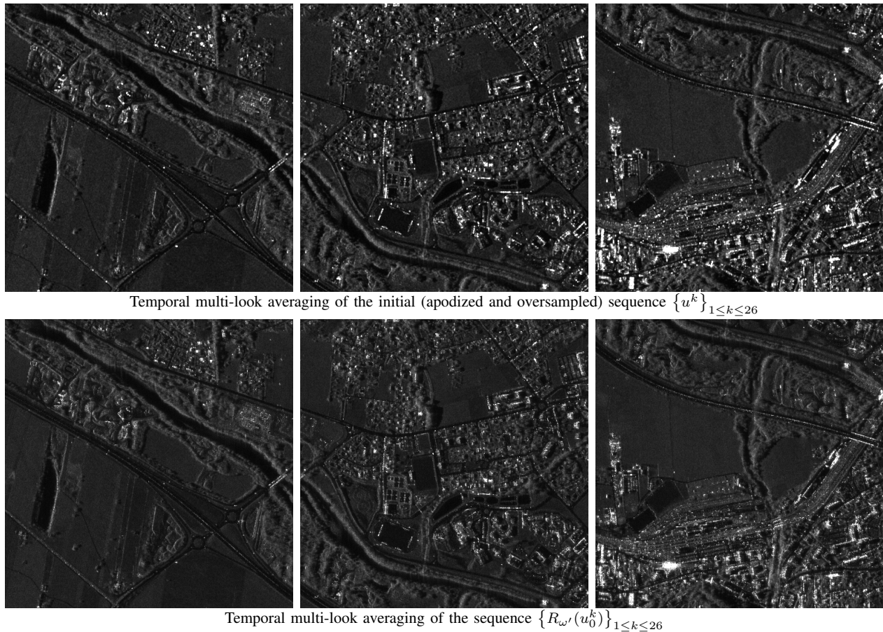
Fig. 16. Temporal multi-look averaging at the initial resolution. First row: several parts of the temporal multi-look averaging computed from twenty-six TerraSAR-X images \{u^k\}_{1 \leq k \leq 26} (used as provided by the spatial agency, i.e., undergoing apodization and oversampling with factors M/m \approx 1.10 and N/n \approx 1.28 in the range and azimuth directions). Second row: the temporal multi-look averaging of the sequence \{R_{\omega'}(u_0^k)\}_{1 \leq k \leq 26} , where \{u_0^k\}_{1 \leq k \leq 26} denotes the pseudo-raw sequence (with spatial domain \omega of size m \times n ) associated to \{u^k\}_{1 \leq k \leq 26} , and \omega' is defined in (25). We can see that using R_{\omega'} yields an efficient resampling of the pseudo-raw sequence since it benefits from the improved level of details of the pseudo-raw sequence (due to the absence of apodization) without suffering from undesirable sidelobe effects in the vicinity of the strong targets.
