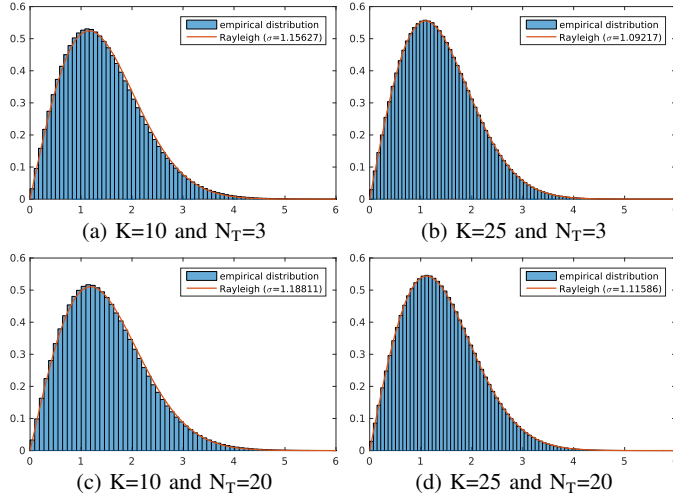
Fig. 9. Distribution of \{R_x^{u_0}(k, \ell)\}_{(k, \ell) \in \omega} in \mathcal{H}_0 . We display the empirical histogram of the sequence \{R_x^{u_0}(k, \ell)\}_{(k, \ell) \in \omega} computed from a 5000 \times 5000 -sized sample u_0 of \mathbf{u}_0 \sim \mathcal{H}_0 using different settings of the parameters K and N_T in Algorithm 2. We can see that those histograms can be well fitted by some Rayleigh probability density functions of the type x \mapsto (x/\sigma^2) \exp(-x^2/(2\sigma^2)) whose parameter \sigma , estimated from \{R_x^{u_0}(k, \ell)\}_{(k, \ell) \in \omega} by mean of a maximum likelihood approach, depends on the setting of (K, N_T) . The same observations hold for the sequence \{R_y^{u_0}(k, \ell)\}_{(k, \ell) \in \omega} . The Rayleigh approximation seems even more accurate for large values of K , as can be observed by comparing (a) to (b) or (c) to (d). The choice K = 25 used in our sidelobe suppression method leads to empirical distributions displayed in (b) and (d) that are still well approximated by a Rayleigh distribution, with a slightly heavier tail than that of the Rayleigh distribution. Therefore, we can consider that Assumption 1 is approximately satisfied, although not rigorously exact.
