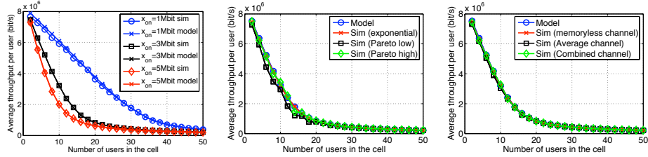
Fig. 2. Performance validation for the three scheduling policies with \bar{x}_{on} = 3 Mbits and \bar{t}_{off} = 3 s.
