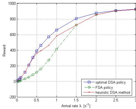
Fig. 4. Operator reward obtained with optimal DSA policy, heuristic DSA and FSA.
