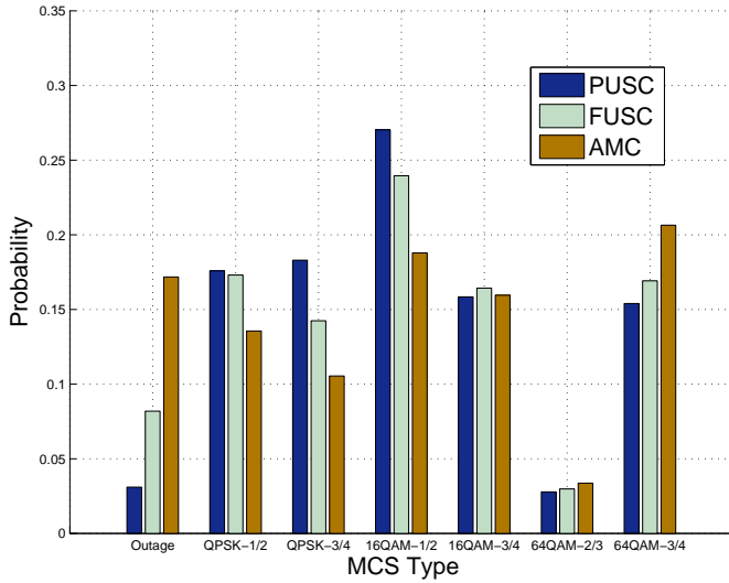
Fig. 5. Comparison of MCS probabilities with PUSC, FUSC and AMC.
