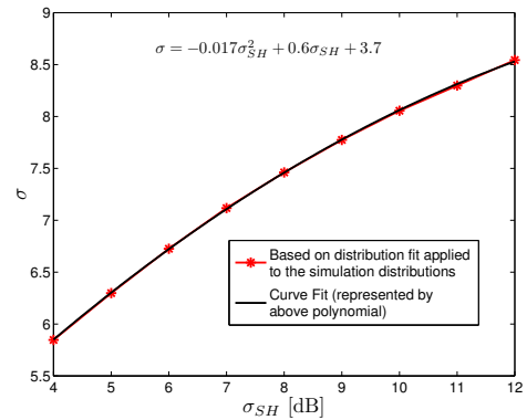
Fig. 7. Scale parameter \sigma of GEV distribution versus \sigma_{SH} for R = 1500 m, P_{Tx} = 43 dBm and reuse 3 \times 3 \times 3 .
