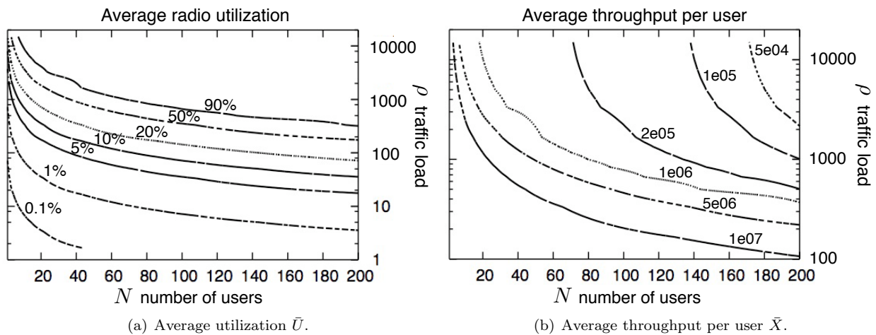
Figure 1.10: Performance graphs
