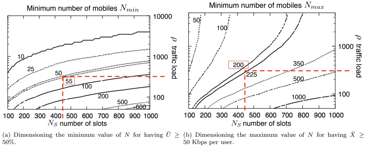
Figure 1.11: Dimensioning graphs
