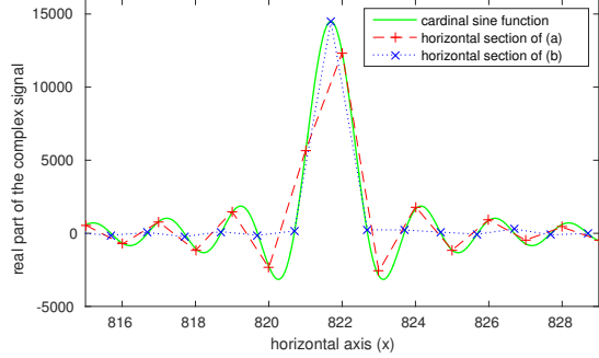
Fig. 3. Resampling targets at the subpixellic scale. We display in (a) the modulus of the pseudo-raw image u_0 in the vicinity of a strong target. We display in (b) and (c) the modulus of the image u_0 resampled by means of a translation of vector t = (0.3, 0) and t = (0.3, 0.1) respectively, yielding more localized signals. We display in the second row a plot of the real part of an horizontal section of u_0 , yielding the red dashed curve, and we do the same for the resampled signal displayed in (b), yielding the blue dotted curve. The green plain curve represents a pure cardinal sine, that is a function of the type x \mapsto A \operatorname{sinc}(x) where A \in \mathbb{R} . We see that the samples of both red and blue signals match very well with a sampling of the cardinal sine, the same observation holds for the imaginary parts of the considered signals.
