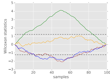
Figure 4. Evolution of the Wilcoxon statistic for 100 samples of 4 quantitative variables. After the 50 th sample, we have modified \Omega with \mu_1 = 3 . The dashed lines indicate the thresholds for detecting a change with a 5% false detection probability.
