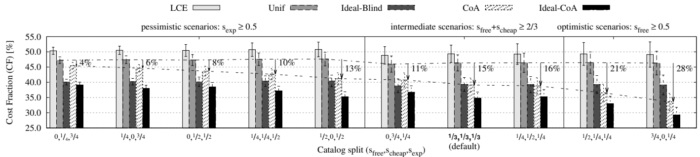
Figure 11. Impact of the catalog split: ( s_{free}, s_{cheap}, s_{exp} ) represent the probability that a content is retrievable through the free, cheap or expensive link, respectively. Arrows indicate the saving achieved by CoA over Unif.
