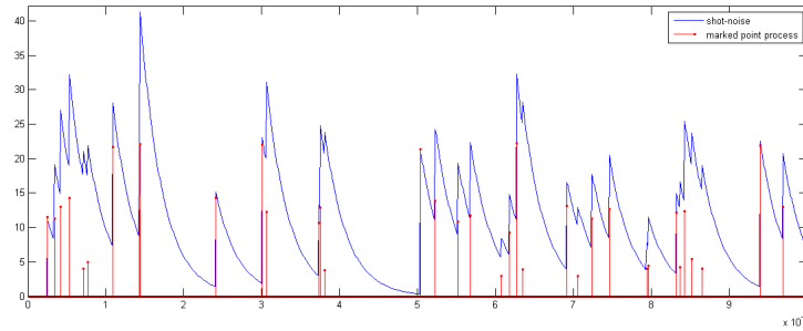
Figure 1: Simulated Shot-Noise
