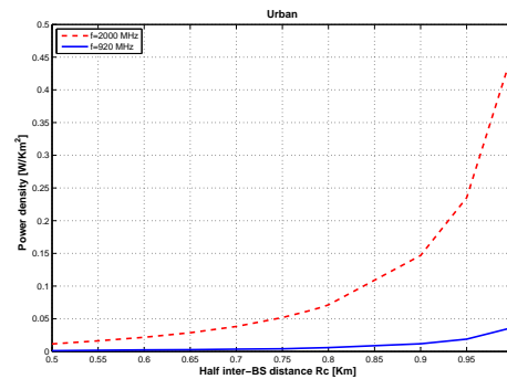
Figure 4. Power density vs. half inter-BS distance.
