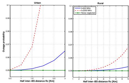
Figure 3. Outage probability vs. half inter-BS distance.
