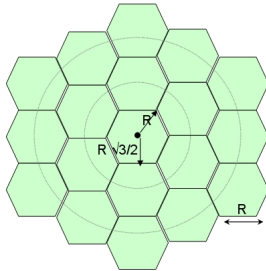
Fig. 1. Hexagonal network of study.
