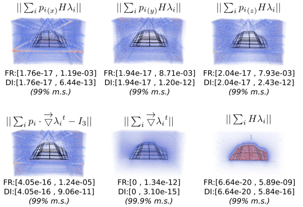
Fig. 4 Validation based on a manufactured solution (group of rigid transformations) for the 3D case. The violation of the correctness conditions (from transparent blue, low values, to opaque red, high value) is measured on each vertex of a 100^3 voxel grid. The full value range (FR) is given below each image while only the 99% most significant samples are displayed (DI). Size of the diagonal of the domain: \sim 600 .
