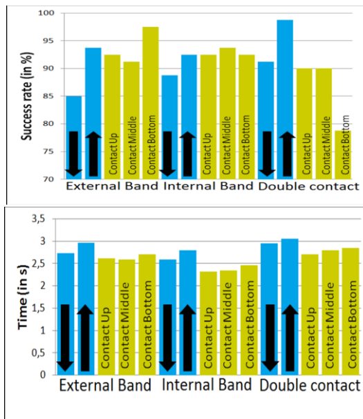
Figure 7: Mean correct recognition rate (top) and mean TtC (bottom) with the gesture vocabulary in eyes-free mode.
