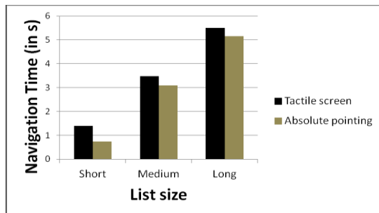
Figure 10: Navigation time depending on list size
