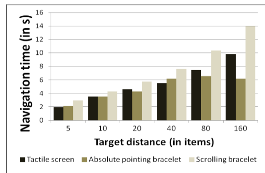
Figure 9: Navigation time depending on target distance for each technique.
