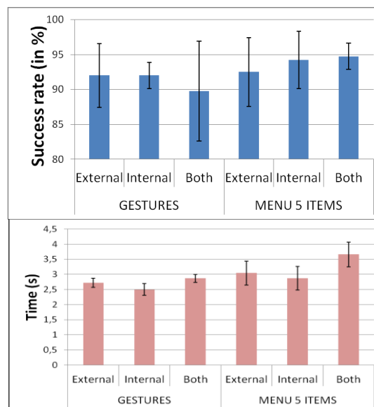
Figure 6: Mean correct recognition rate (up) and mean total trial completion time (down) for both the gesture and the audio menu techniques. Error bars show standard deviations.
