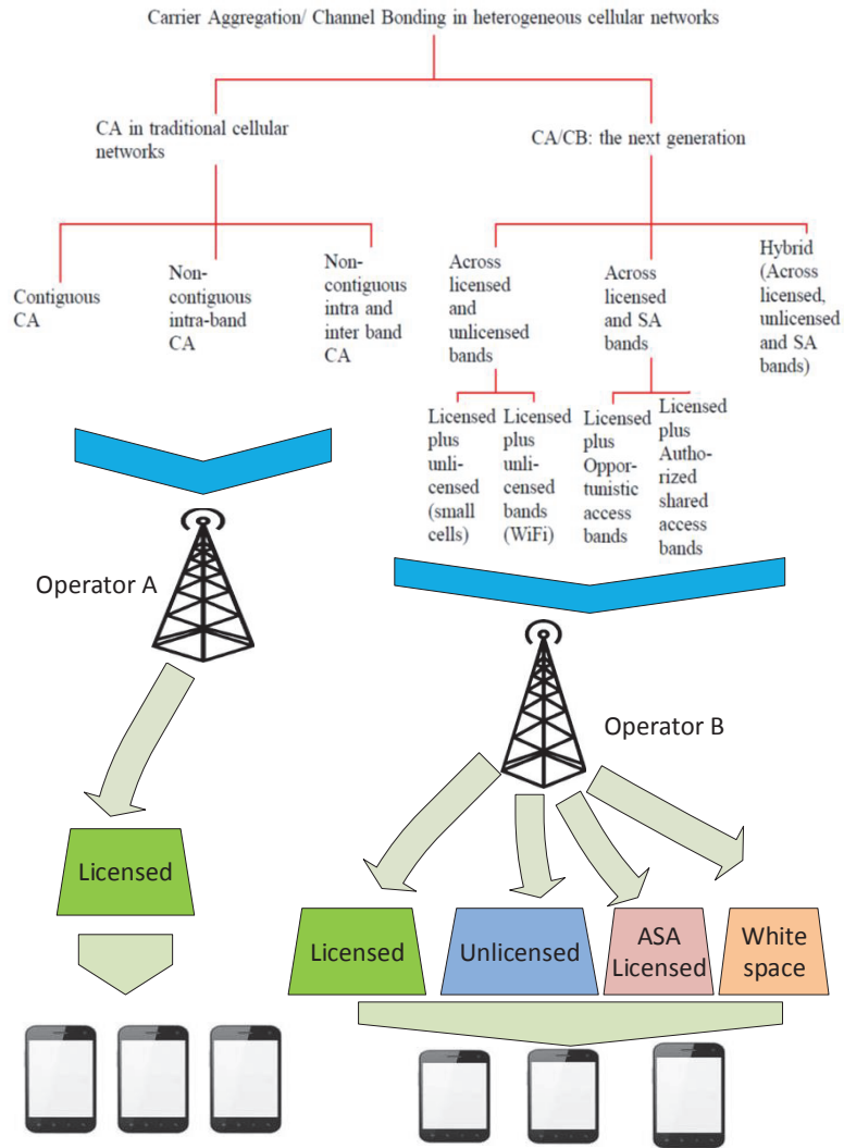
Fig. 1. CA/CB taxonomy and different spectrum band utilization for aggregation in traditional and next generation networks.
