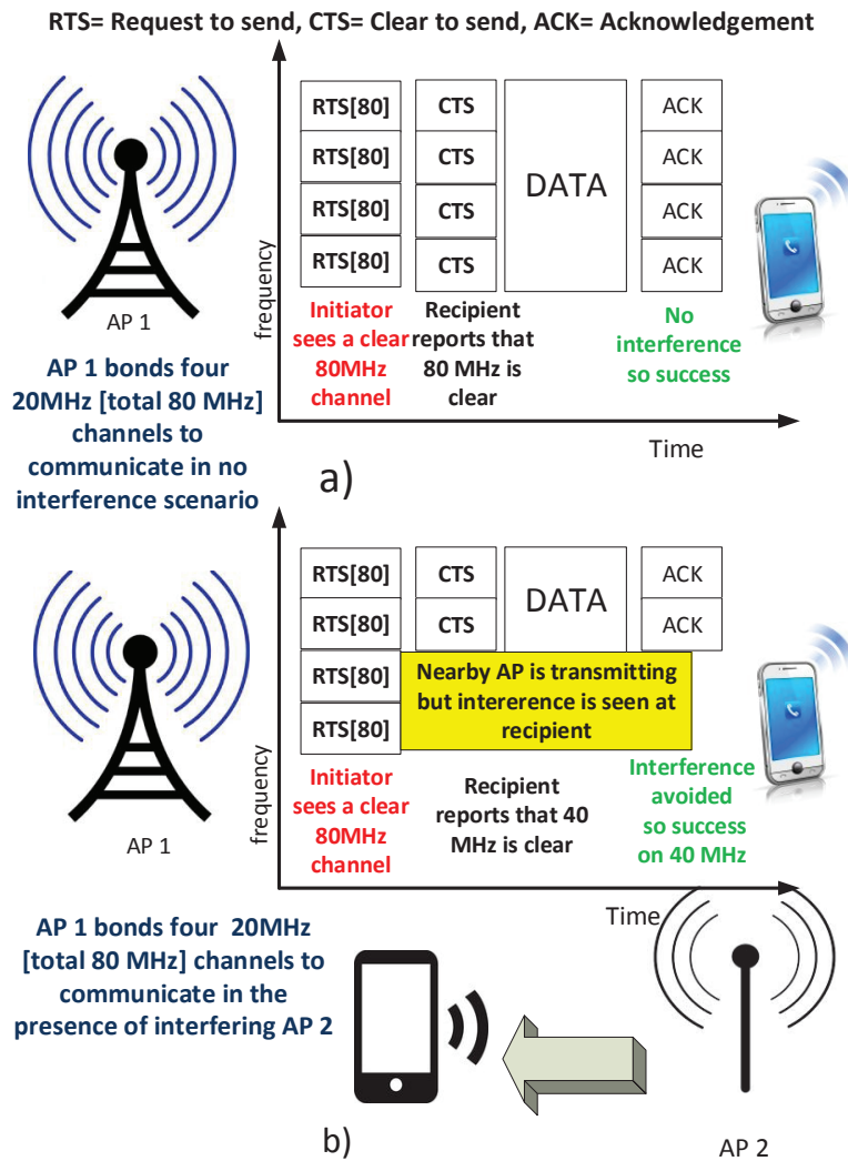
Fig. 4. Examples of enhanced RTS/CTS channel bonding protocol: a) When access point (AP) 1 is bonding to communicate in the absence of interference; and b) When AP 1 is bonding to communicate in the presence of interference.
