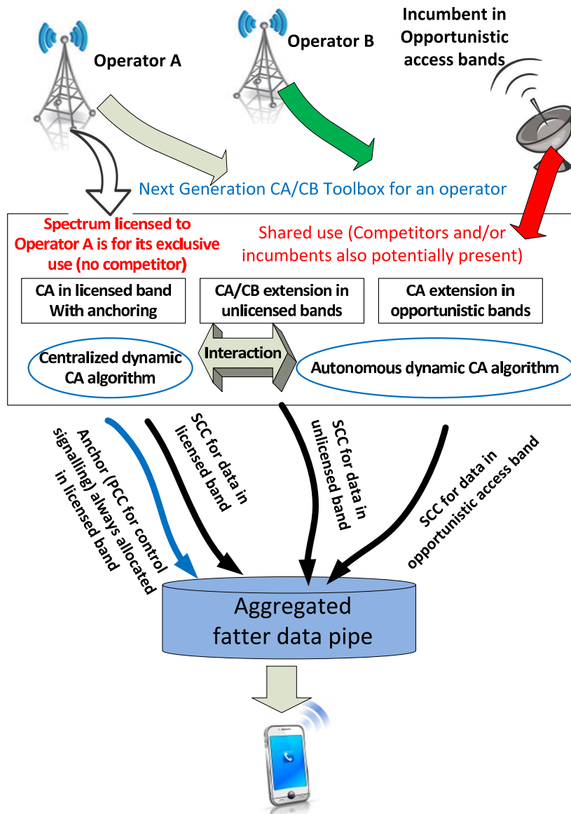
Fig. 2. Next generation CA/CB toolbox. PCC denotes primary component carrier and SCC denotes secondary component carrier.
