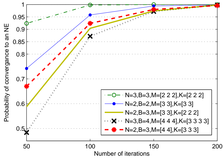
Fig. 3. Convergence probability of the randomized best response dynamic to an NE for different scenarios. K shows the number of carriers in each band and M shows the number of carriers that each user can aggregate.
