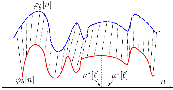
Fig. 3. Example of association of two sequences by Dynamic Time Warping.
