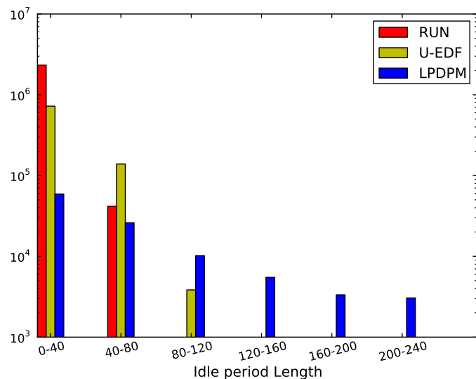
Fig. 5. Distribution of idle periods lengths
