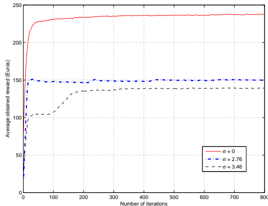
Figure 4. Average reward versus the number of iterations.
