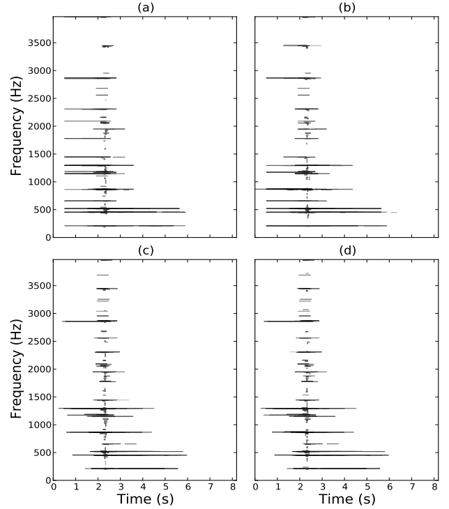
Fig. 2. Energy distributions of a bell sound decomposed by MP and LOMP algorithms. Left: original signal decomposition at 20 dB of SRR with 8 MDCT basis with MP (a) and LOMP (c). Right: decomposition of the same signals shifted in time by 100 samples with MP (b) and LOMP (d).
