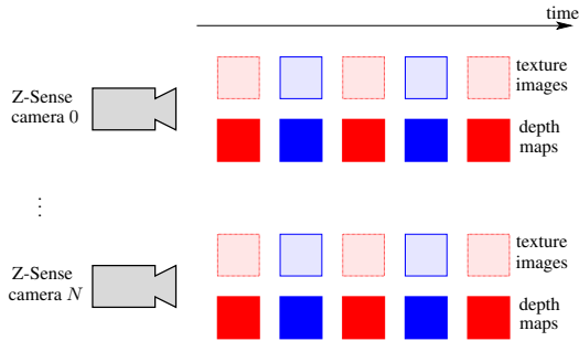
Fig. 2. The frame repartition in time-view domain used in this paper (GOP size equal to 2). The KFs are in red, while the WZs are in blue. The texture images and the depth maps are independently coded.
