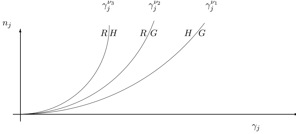
FIGURE 1. Pairwise comparisons of the rates of convergence of \mathbf{S}_{n_j, j}^{(1,1,0)}(G) , \Sigma_{n_j, j}^{(0)} + \Sigma_{n_j, j}^{(1)}(R) and \Sigma_{n_j, j}^{(2)}(H) in the plane \gamma_j versus n_j .
