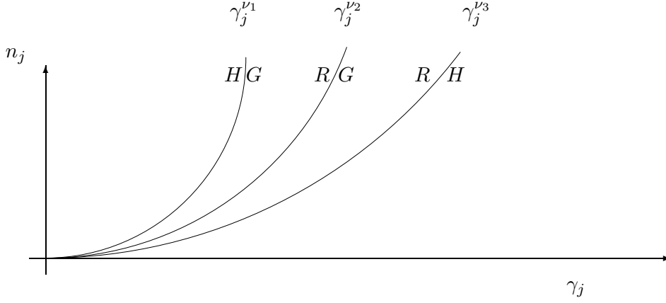
FIGURE 2. Domains of convergence for Theorem 3.3
