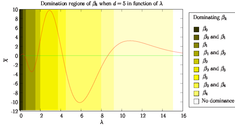
FIGURE 7. Behavior of \chi with respect to \lambda .
