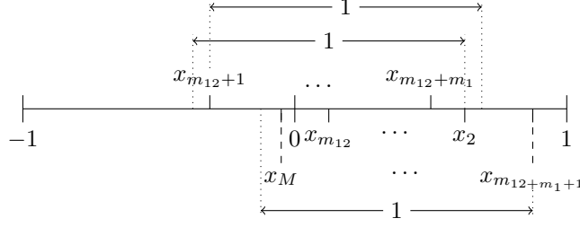
FIGURE 6. Example of relative positions of the points
